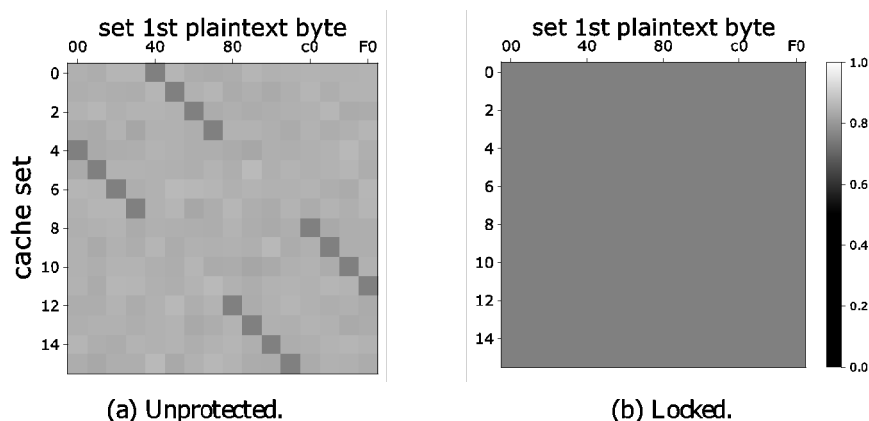
Figure 1: For a given secret key (0x42), the hit rate for each cache set (on the Y-axis) is shown relative to the first byte of the plaintext (X-axis). In the unprotected case, discernible patterns allow information about the secret key to be recovered. In the locked case, the hit rate remains constant, making the attack ineffective. (Figure adapted from [1]).
