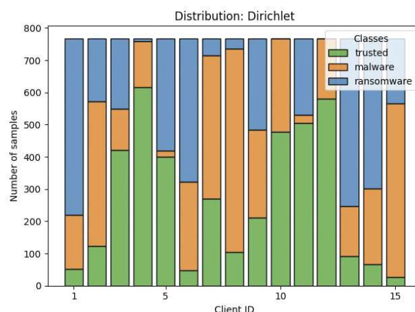
Figure 1: The Dirichlet distribution obtained among 15 different clients.
